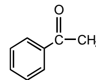
acetophenone
