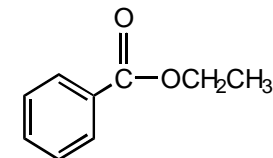
ethyl benzoate
